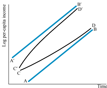
Figure 4.2. Conditional convergence.
