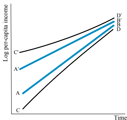
Figure 4.3. Parametric convergence.
