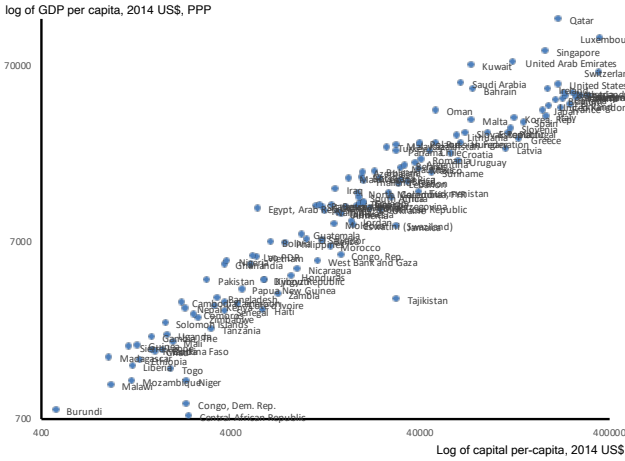
Figure 3.2. Log capital per-capita and log income per-capita, 2014. Source: World Bank Wealth Accounts database and World Development Indicators
