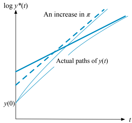
Figure 3.8. A change in \pi has growth effects.
