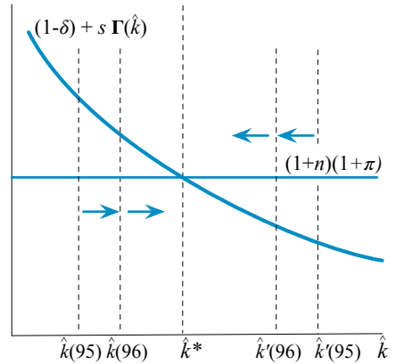
Figure 3.5. The Solow model with technical change.
