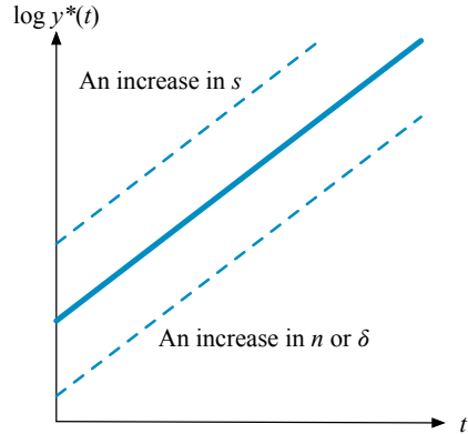
Figure 3.7. s , n and \delta have level effects.
