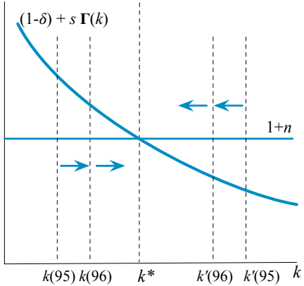
Figure 3.4. Growth dynamics in the Solow model.
