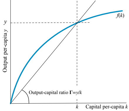
Figure 3.3. The production function in per-capita form.
