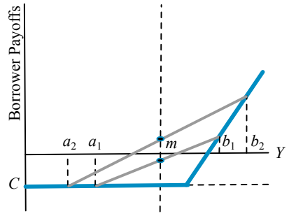
Figure 19.4. A higher interest rate degrades the borrower pool.
