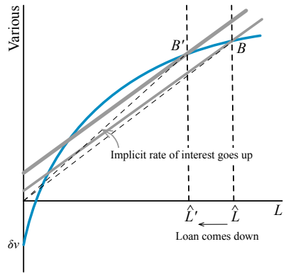
Figure 19.11. Change in lender profit.
