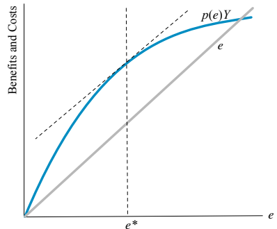
Figure 19.5. Effort under self-financing.
