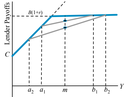
Figure 19.3. Net payoffs to lender.
