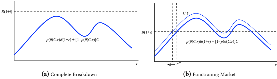
Figure 19.13. Equilibrium Interest Rate With Collateral C .
