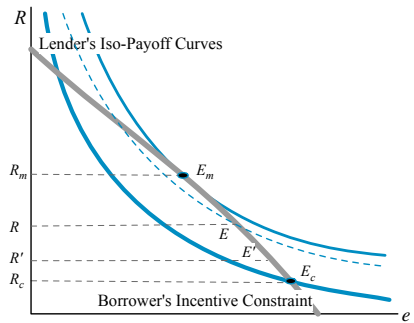
Figure 19.7. Repayment and Effort.
