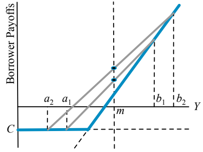
Figure 19.2. Net payoffs to borrower.
