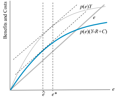
Figure 19.6. Debt and effort.
