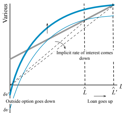
Figure 19.12. Change in outside options.
