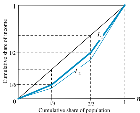
Figure 10.4. The transfers principle and the Lorenz criterion
