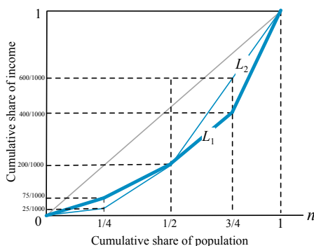
Figure 10.5. Ambiguous comparisons: A Lorenz crossing.
