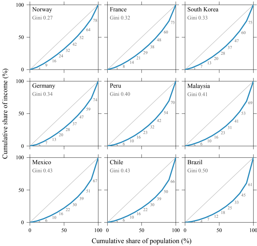
Figure 10.6. Lorenz curves for nine countries, ordered by increasing inequality. The figures along each curve are cumulative percentage shares of income at each decile. Source: World Bank Poverty and Inequality Platform (PIP), most recent survey available for each country as of 2026, spanning 2021–2024. All nine estimates are income-based rather than consumption-based, and the income concept is household disposable income — that is, income measured after taxes and transfers.
